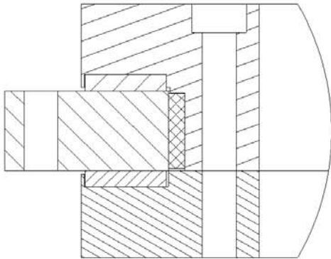
DETAIL B SCALE 3 : 4
