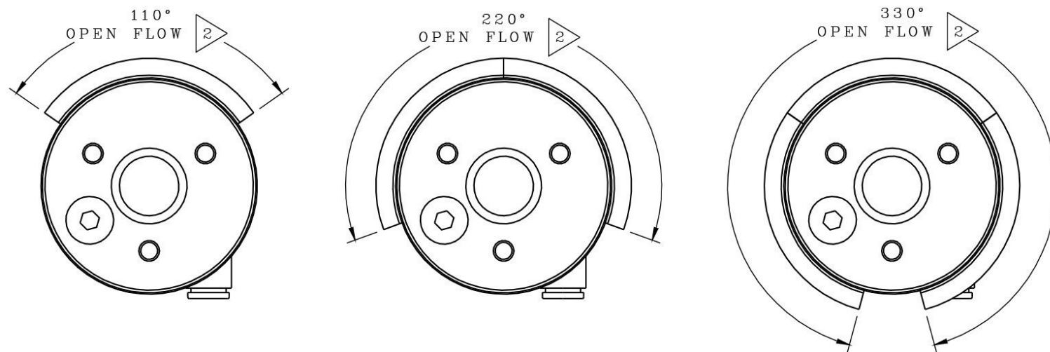
VIEW B-B (WITH VARYING WRAP ANGLES) SCALE 5:8
