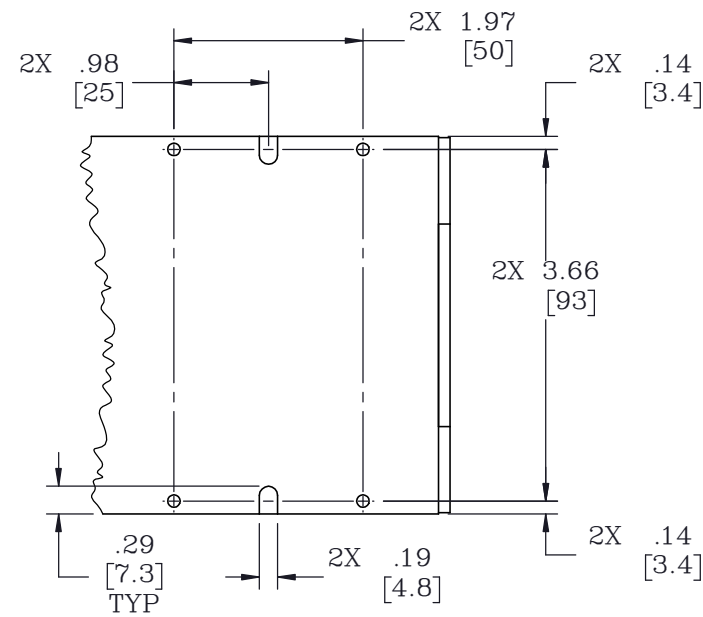
DETAIL A (4X) SCALE 1:2
